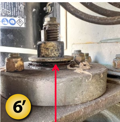
Tapered Bearing
