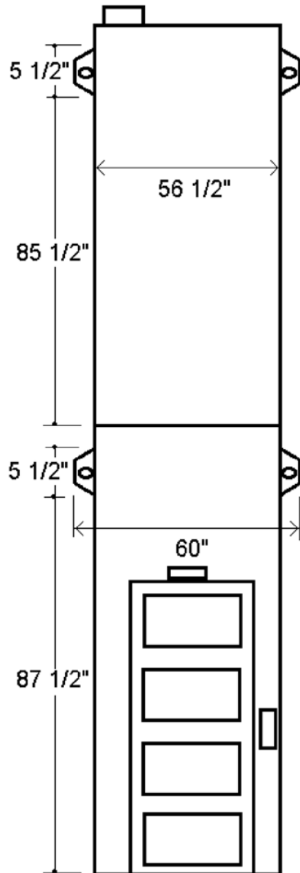
FRONT VIEW
